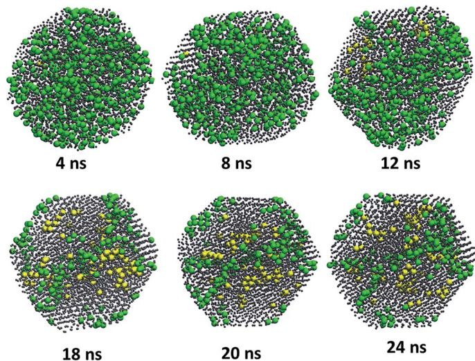
Fig. 10 Crystal structure analysis of the gold nanoparticles on the basis of local bond order parameter analysis. Green and yellow colors represent atoms with hcp and fcc structures, respectively. Gray color represents atoms in the disordered state.
