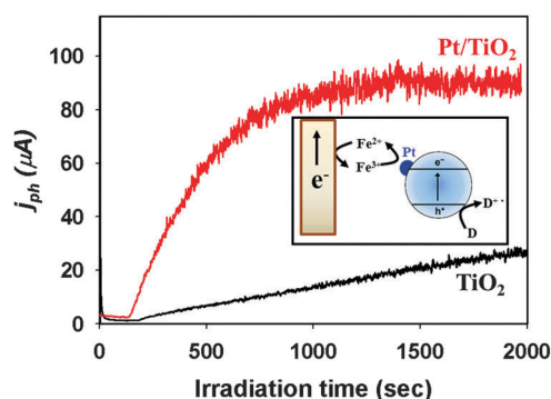
Fig. 3 Comparison of \text{Fe}^{3+} -mediated photocurrents collected on a Pt electrode for \text{TiO}_2 and \text{Pt}/\text{TiO}_2 . The inset shows the current collection on an inert Pt electrode immersed in an UV-illuminated \text{Pt}/\text{TiO}_2 suspension. Adapted with permission from ref. 150 (Copyright 2014 American Chemical Society).
