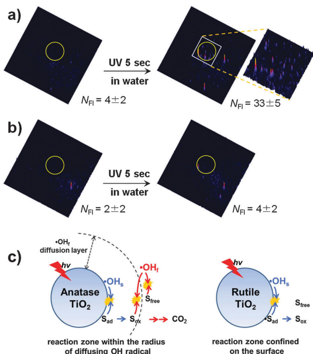
Fig. 2 (a and b) Fluorescence images of free hydroxyl radicals ( \bullet\text{OH} ) that migrated through a gap from the UV-illuminated \text{TiO}_2 (a: anatase, b: rutile) to HPF-coated cover glass. The \text{TiO}_2 /water system with silanol-modified HPF (3'-(p-hydroxyphenyl)fluorescein) was compared before (left) and after (right) UV irradiation for 5 s. The diffusion gap is 7.5 \mu\text{m} . The UV irradiation region is inside the yellow circle in the images. NFI indicates the number of fluorescence signals. The size of the image is 50 \times 50 \mu\text{m} . (c) Illustration of OH-radical-mediated photocatalysis on anatase and rutile. Reprinted with permission from ref. 74 (Copyright 2014 Wiley-VCH Verlag GmbH & Co. KGaA, Weinheim).
