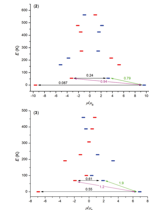
Fig. 4 The ab initio computed magnetization blocking barrier for complexes 2 and 3. The thick blue/red bars indicate the Kramers doublets (KDs) as a function of magnetic moment. Green lines indicate the magnetization reversal mechanism. The magenta lines show the possible pathway of the Orbach process. The black lines represent the presence of QTM/TA-QTM between the connecting pairs.
