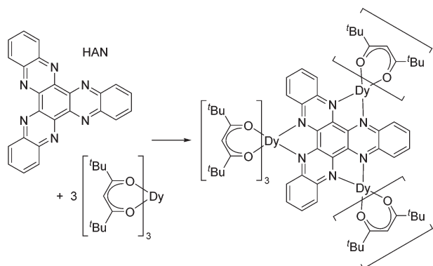
Scheme 1 Synthesis of [\{(thd)_3Dy\}_3HAN] ( 1 ).
