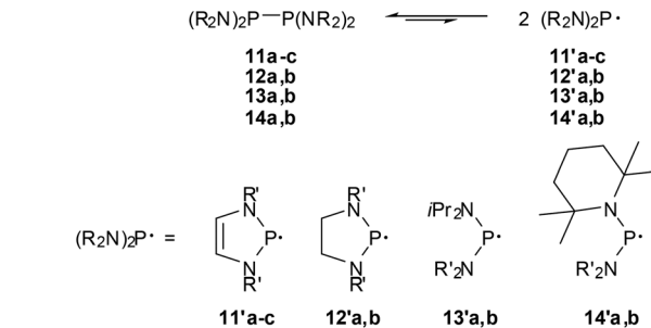
Scheme 13 P–P bond dissociation equilibria for tetraamino-diphosphines (R' = t Bu ( 11a ), 2,6-Me 2 C 6 H 3 ( 11b ), 2,6- i Pr 2 C 6 H 3 ( 11b , 12a ), 2- t Bu 2 C 6 H 4 ( 12b ), i Pr ( 13a , 14b ), SiMe 3 ( 13b ), Et ( 14a )).
