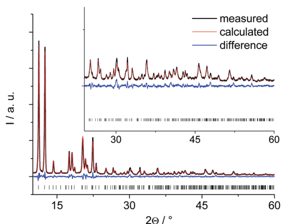
Fig. 1 The Rietveld plot for the anhydrous Al-MIL-53-ADP-np. The black line is the experimental data, the red line is the fit and the blue line the difference curve. Vertical bars mark the Bragg reflection positions.
