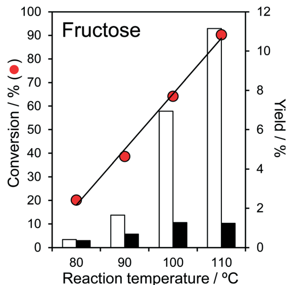
Fig. 3 Aqueous phase conversion of glucose and fructose over parent PNA and corresponding yields of 5-HMF (white) and fructose/glucose (black) as a function of reaction temperature: 0.1 g glucose or fructose, 0.1 g PNA, 20 cm 3 water, 6 h.
