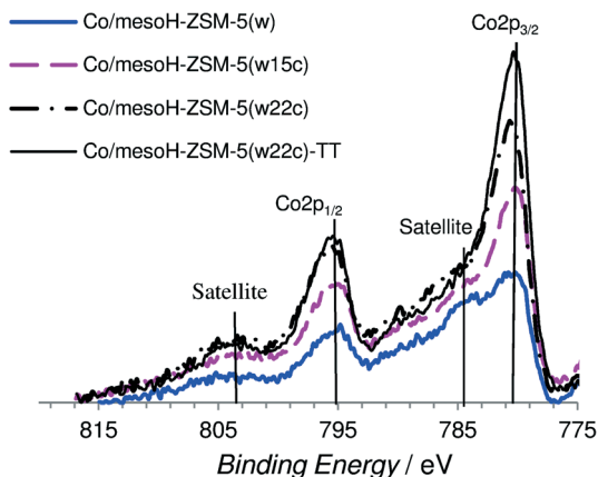
Fig. 6 XPS spectra (Co 2p region) of the different Co-supported catalysts.
