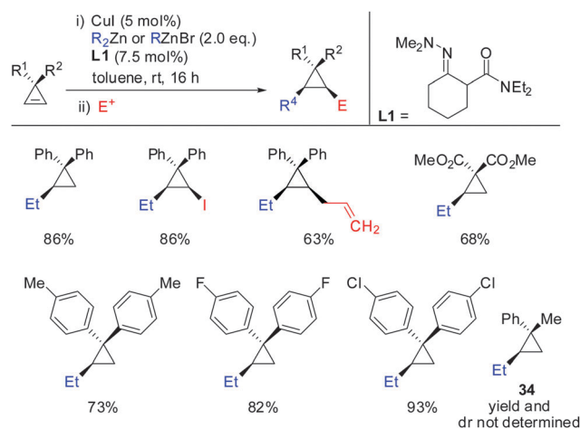
Scheme 28 Copper-catalysed carbozincation reaction of non-functionalized cyclopropenes.
