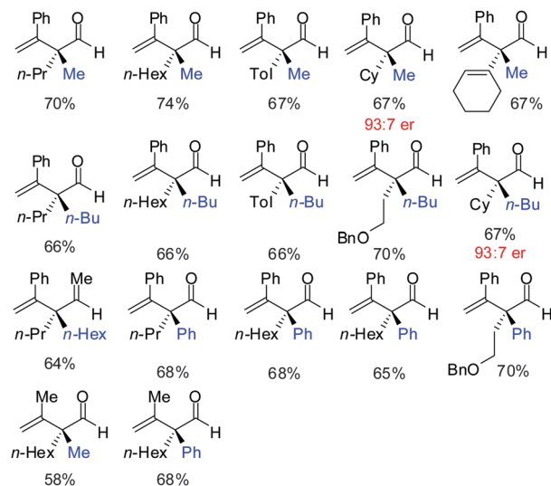
Scheme 38 Carbometalation-oxidation-elimination sequence.
