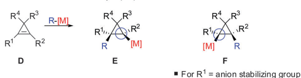
Scheme 9 Regioselectivity of carbocupration reactions.
