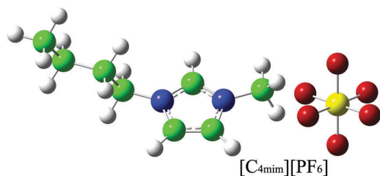
Fig. 1 3-Butyl-1-methyl-1H-imidazolium hexafluorophosphate, [\text{C}_4\text{mim}][\text{PF}_6] , green = C, white = H, blue = N, red = F, yellow = P.
