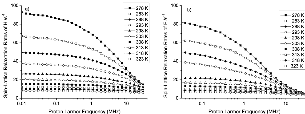
Fig. 2 R_1 -NMRD profiles of R_{1,\text{H},\text{EXP}}(\omega) (a) and R_{1,\text{F},\text{EXP}}(\omega) (b) at temperatures ranging from 278 K to 323 K. Best fit parameters obtained from the NMRD analysis are given in Tables 2 and 3.
