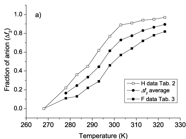
Fig. 3 The temperature dependence of the relaxation rates in Tables 2 and 3 of H(R_1(\max)) (a) and F(R_1(\max)) (b) versus the 100/T , are displayed. H and F R_1 -NMRD profiles have the same temperature dependence. Also the temperature dependence of the correlation time ( \tau_{c,2} = \tau_{c,2} ) and R_1(\text{slow}) = R_1(\tau_{c,2}) of Tables 2 and 3 is displayed.
