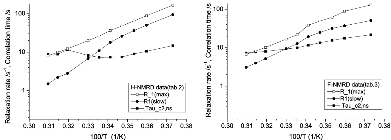
Fig. 3 The temperature dependence of the relaxation rates in Tables 2 and 3 of H(R_1(\max)) (a) and F(R_1(\max)) (b) versus the 100/T , are displayed. H and F R_1 -NMRD profiles have the same temperature dependence. Also the temperature dependence of the correlation time ( \tau_{c,2} = \tau_{c,2} ) and R_1(\text{slow}) = R_1(\tau_{c,2}) of Tables 2 and 3 is displayed.
