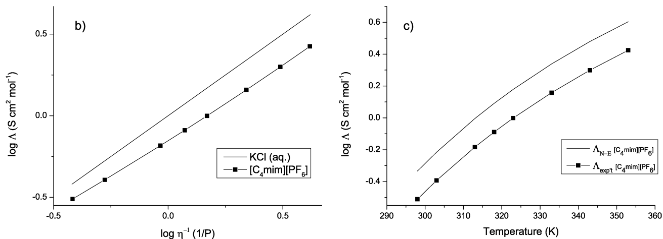
Fig. 4 (a) Free ion fractions of [C_4mim]^+ and [PF_6]^- ions, in the range T = 268\text{--}323 K. (b) Corresponding Walden plot, (c) corresponding N-E plot.
