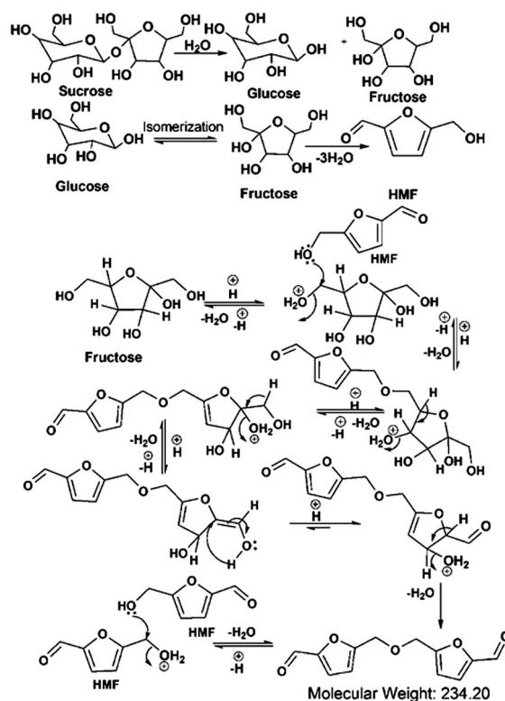
Scheme 2 Mechanism of formation of the HMF derivative in carbon dots using sucrose and \text{H}_3\text{PO}_4 .
