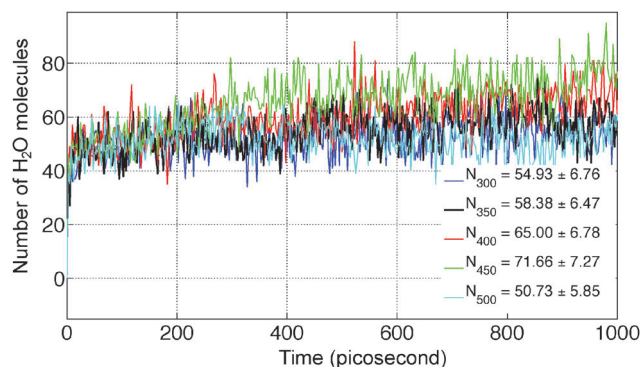
Fig. 12 Dehydration kinetics of \text{MgCl}_2\cdot 2\text{H}_2\text{O} in a 2D-periodic slab of 44.3 \times 1000 \times 21.9 Å upto 1 nanosecond using ReaxFF-MD simulations. N_T is average number of \text{H}_2\text{O} molecules escaping from the slab at temperature T .
