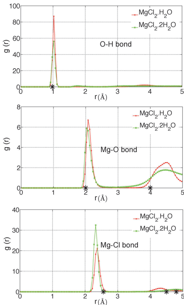
Fig. 10 Radial distribution functions of O–H, Mg–O, and Mg–Cl bond in \text{MgCl}_2\cdot\text{H}_2\text{O} and \text{MgCl}_2\cdot 2\text{H}_2\text{O} obtained with newly developed ReaxFF parameters of \text{MgCl}_2 hydrates at 300 K. The represents the corresponding distance in the experimental unit cell. 43,44
