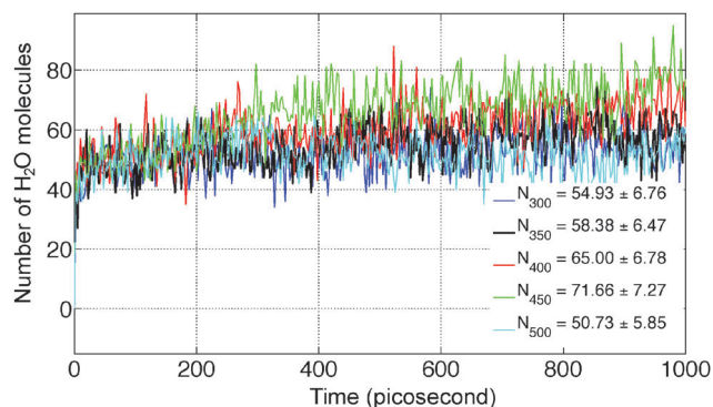
Fig. 12 Dehydration kinetics of \text{MgCl}_2\cdot 2\text{H}_2\text{O} in a 2D-periodic slab of 44.3 \times 1000 \times 21.9 \text{ \AA} upto 1 nanosecond using ReaxFF-MD simulations. N_T is average number of \text{H}_2\text{O} molecules escaping from the slab at temperature T .
