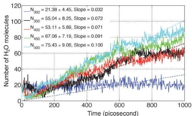
Fig. 11 Dehydration kinetics of \text{MgCl}_2\cdot\text{H}_2\text{O} in a 2D-periodic slab of 26.8 \times 21.8 \times 1000 \text{ \AA} upto 1 nanosecond using ReaxFF-MD simulations. The solid lines represent the kinetics from ReaxFF-MD simulations while the dashed lines of the same color represent a linear fit to estimate the dehydration rate. N_T is average number of \text{H}_2\text{O} molecules escaping from the slab at temperature T .
