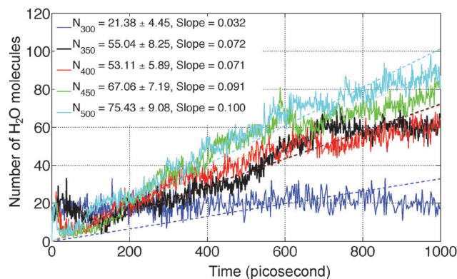
Fig. 11 Dehydration kinetics of \text{MgCl}_2\cdot\text{H}_2\text{O} in a 2D-periodic slab of 26.8 \times 21.8 \times 1000 Å upto 1 nanosecond using ReaxFF-MD simulations. The solid lines represent the kinetics from ReaxFF-MD simulations while the dashed lines of the same color represent a linear fit to estimate the dehydration rate. N_T is average number of \text{H}_2\text{O} molecules escaping from the slab at temperature T .
