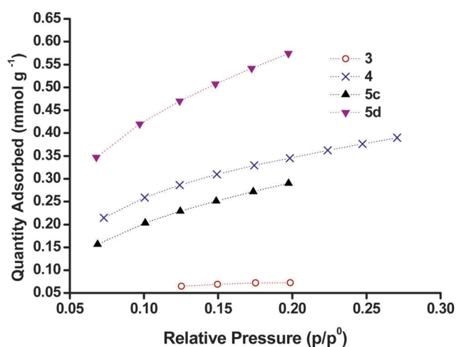
Fig. 6 Kr gas adsorption for NiO films made from NiO films made from sol–gel methods with different block copolymers, 4 (blue) and 3 (brown) and Dyenamo NiO paste and sintered at 350 °C ( 5c , black) and 450 °C ( 5d , purple).
