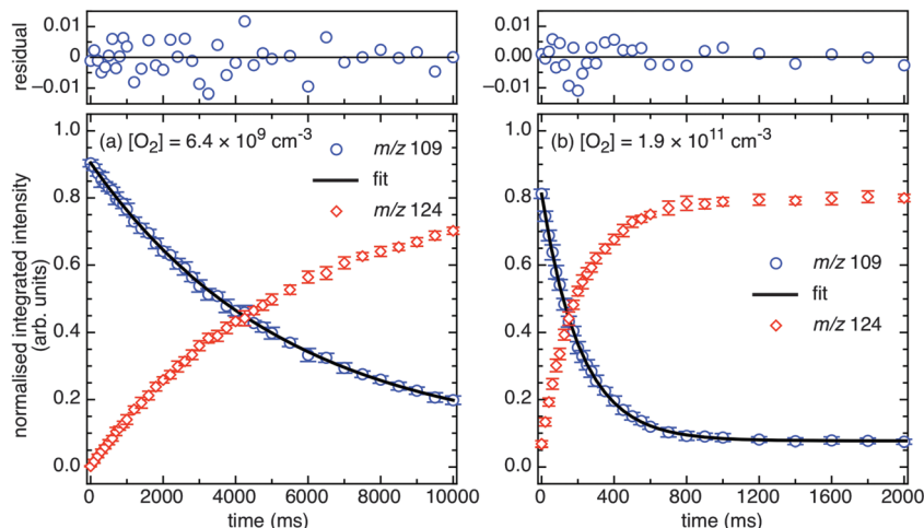
Fig. 5 Kinetic curves for m/z 109 (solid blue circles), from PD of 3-bromo-4-hydroxybenzaminium cations, in reactions with (a) background O_2 ( 6.4 \times 10^9 molecules cm^{-3} ) and (b) increased O_2 ( 1.9 \times 10^{11} molecules cm^{-3} ). Residual plots from the fitting of eqn (1) are provided above. The m/z 124 product data are shown (red diamonds) and track with a rate coefficient in agreement with the m/z 109 decay (within 2\sigma ). Error bars are 1\sigma .
