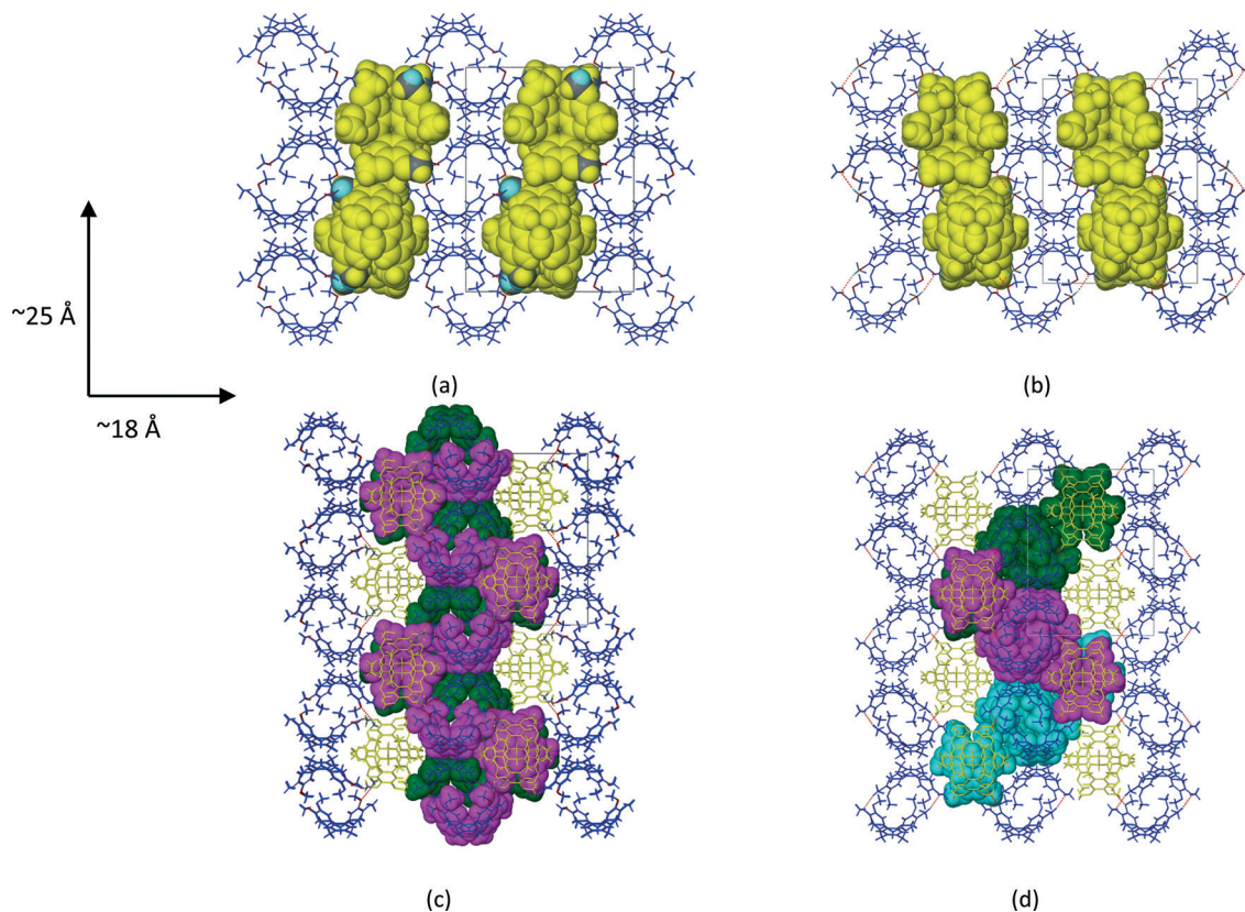
Fig. 2 Packing diagrams of CTV molecules in (a) 1a and (b) 2a with 'stacked' CTV molecules shown in space-filling mode. (c) CTV molecules in 1a and (d) 2a connected by C–H⋯O hydrogen bonding shown in space-filling mode and the same colour. All views are down the \sim 10 Å axis.
