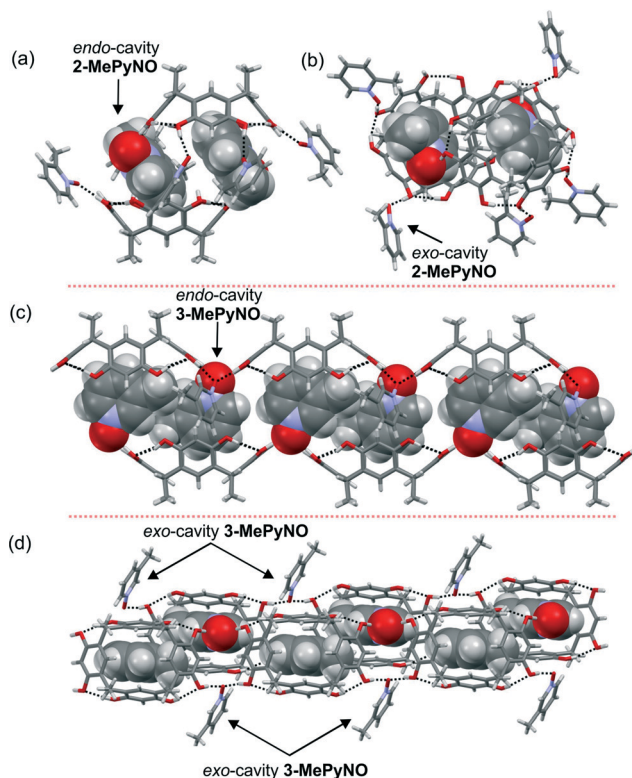
Fig. 2 (a) Side view of the discrete dimeric structure of 2-MePyNO- 1 , and (b) top view showing exo-cavity HB monodentate decorated 2-MePyNO with host 1 . (c) Section of the 1-D polymeric crystal packing in 3-MePyNO- 1 showing endo 3-MePyNO as a bidentate HB acceptor, and the respective (d) side view showing the exo -cavity HB bidentate 3-MePyNO molecules.
