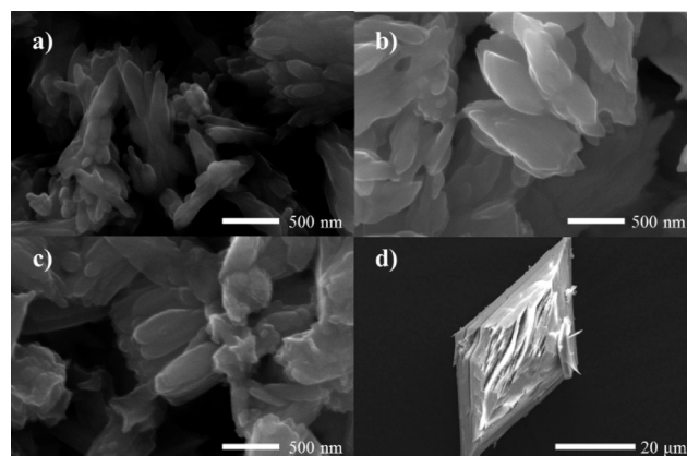
Fig. 2 SEM images of crystals of 1 prepared at room temperature using a reaction solution containing 0.1 M NaOH over a) 0.5 h and b) 16 h, or c) with Na 2 bcppm over 16 h, and d) a conventional preparation over 16 h.
