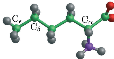
Fig. 4 A norleucine molecule in the conformation belonging to the \beta and \alpha polymorphic forms. The indicated C_\alpha , C_\beta and C_\epsilon are being used in the NEB and steered MD calculations.
