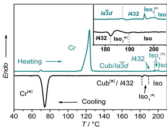
Fig. 1 DSC heating and cooling traces (10 \text{K min}^{-1} ) observed for the complex AB8 . The inset shows the heating and cooling traces for the temperature range of the Iso–Iso 1 [*] –Cub [*] /I432 transitions between 175 °C and 205 °C.
