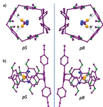
Fig. 2 Crystal structure of compound 2 in CH_2Cl_2 which displays planar chirality. Hydrogens on 2 omitted for clarity. (a) pS - and pR -conformations of 2 in CH_2Cl_2 (top view); (b) (side view). The blue dotted lines indicate the C-H... \pi interactions. Color codes: carbon, purple; hydrogen, orange; oxygen, green; and chlorine, blue.
