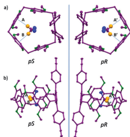
Fig. 2 Crystal structure of compound 2 \cdot CH_2Cl_2 which displays planar chirality. Hydrogens on 2 omitted for clarity. (a) pS - and pR -conformations of 2 \cdot CH_2Cl_2 (top view); (b) (side view). The blue dotted lines indicate the C-H... \pi interactions. Color codes: carbon, purple; hydrogen, orange; oxygen, green; and chlorine, blue.
