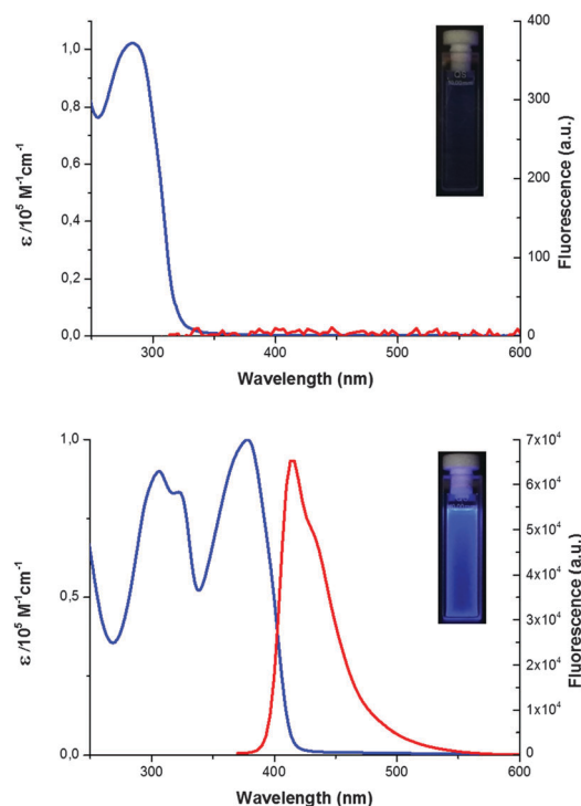
Fig. 3 UV-visible absorption (blue line) and fluorescence (red line) spectra of monomers 2 (top, 10^{-5} M) and 1 (bottom, [RU] = 10^{-5} M, chloroform).
