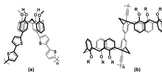
Fig. 1 Representative conjugated polymer adopting macrocycles as backbones.
