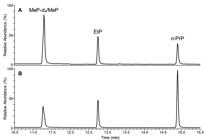
Fig. 1 GC-qMS chromatograms of target screening for methylparaben (MeP), ethylparaben (EtP) and n -propylparaben ( n -PrP) with the internal standard methylparaben- d 4 (MeP- d 4 ). (A) Calibration level 50 \mu\text{g 10 mL}^{-1} and (B) gel sample extract of baby teether no. 3.
