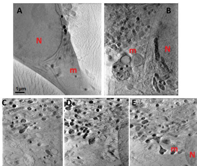
Fig. 3 Soft X-ray microscopy: comparison of two different GBM cells: (a) U87MG and cell line 11ST (b). N-nucleus of cell, m-mitochondria. Virtual slices of a tomogram of one cell isolated from 11ST (c–e).
