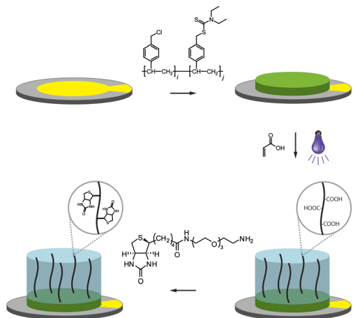
Fig. 1 Fabrication of biotin-functionalized pAAc sensor. Gold-plated QCM crystals were first coated with the photoreactive copolymer PVBD 50.1 , which was subsequently subjected to poly(acrylic acid) brush formation under UV irradiation. Final coupling of (+)-biotinyl 3,6,9-trioxaundecanediamine to the carboxylic acid groups yielded functionalized QCM sensor surfaces of three-dimensional character.
