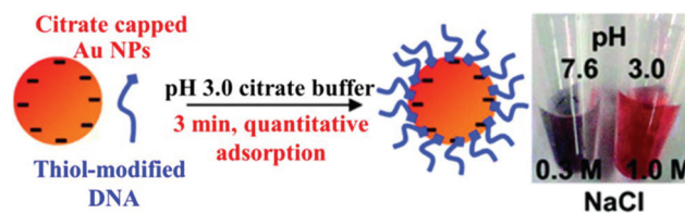
Fig. 2 Schematic illustration of attaching negatively charged thiolated DNA to negatively charged Au NPs using the low pH assisted method. Reprinted with permission from ref. 48. Copyright 2012, American Chemical Society.
