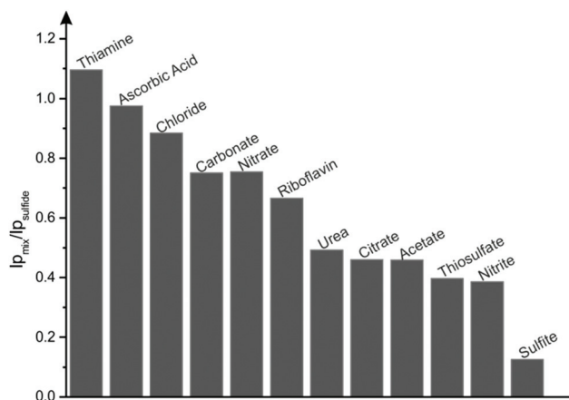
Fig. 3 LSV peak current ratio of sulfide (2 mM) in the presence of co-existent interferents ([sulfide]:[interferents] 1:20) at CuSPE sensor. Note that concentration of riboflavin is 0.2 mM as it is sparingly soluble in aqueous solutions.
