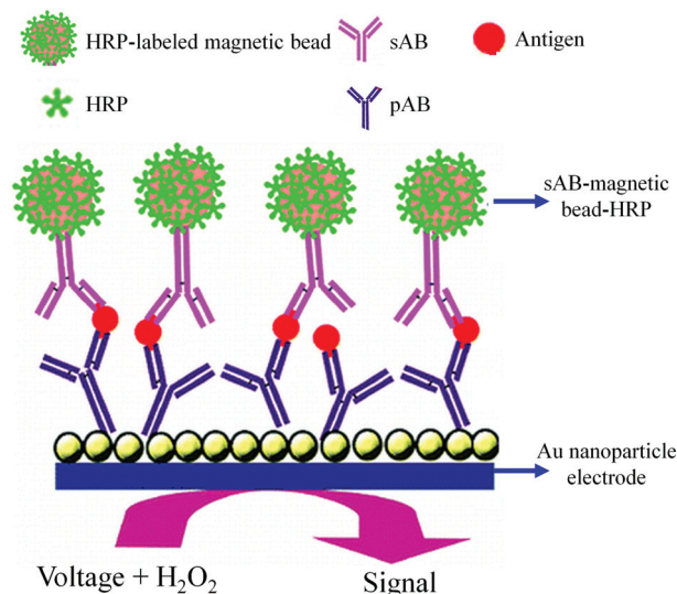
Fig. 8 AuNP based electrochemical immunosensor (adapted with permission from ACS Nano , 2009, 3, 585–594. Copyright (2009) American Chemical Society).
