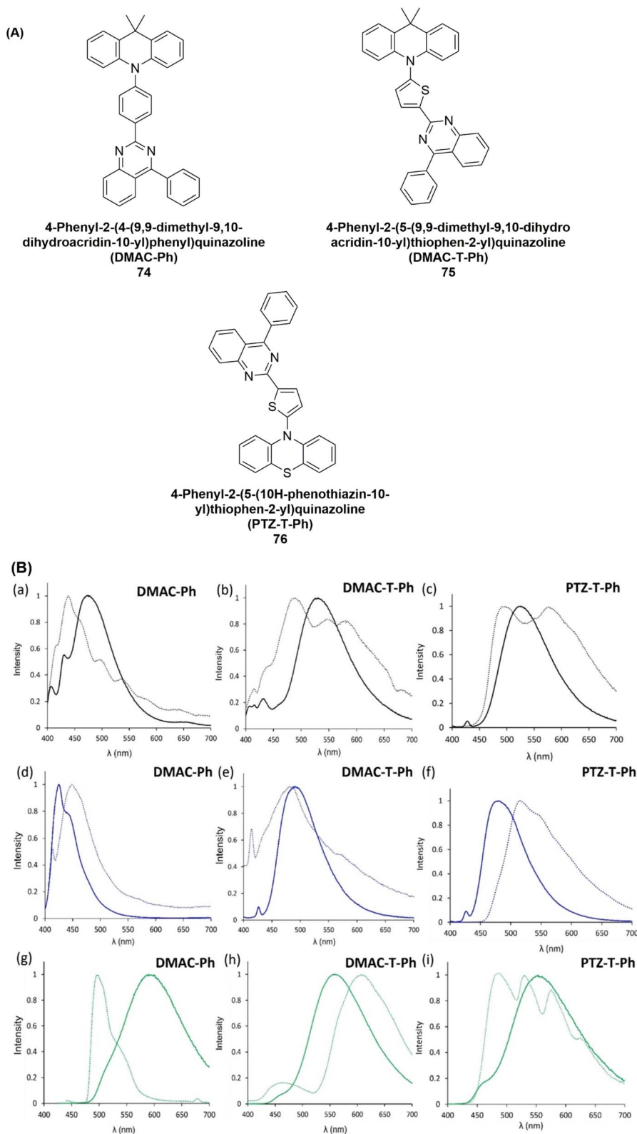
Fig. 26 (A) Chemical structure of DMAC-Ph ( 74 ), DMAC-T-Ph ( 75 ), and PTZ-T-Ph ( 76 ). (B) Normalized emission spectra of DMAC-Ph, DMAC-T-Ph, and PTZ-T-Ph recorded at 25 °C (solid lines) and 77 K (dotted lines) in (a–c) toluene, (d–f) n -heptane, and (g–i) Me-THF. Excitation wavelengths correspond to the respective absorption maxima. Reproduced from ref. 105 with permission from Wiley, Copyright © 2025, under the terms of the CC (BY-NC) 3.0 license.
