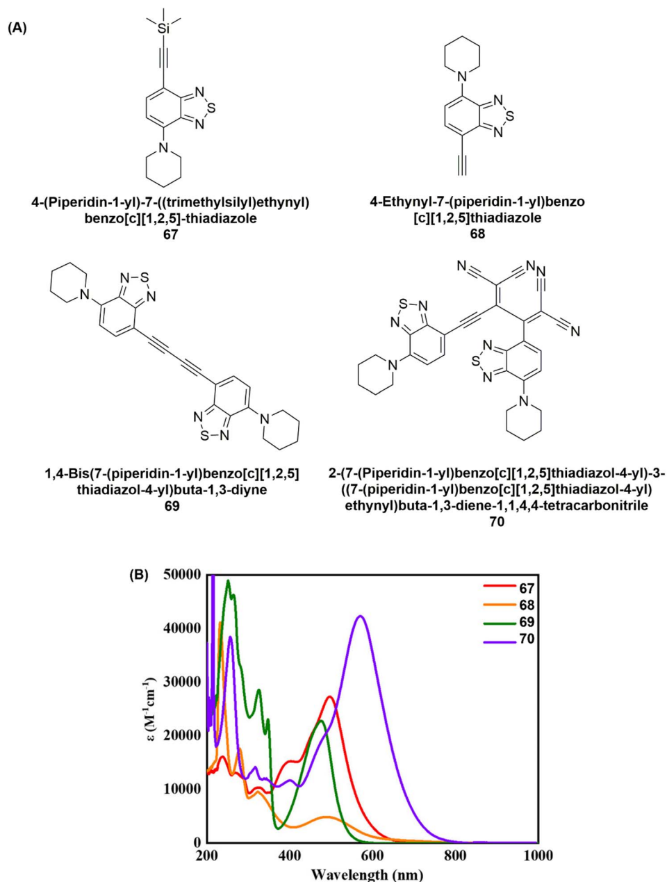
Fig. 24 (A) Chemical structure of TCBD derivatives 67–70. (B) UV-vis absorption spectra of TCBD derivatives 67–70 recorded in \text{CH}_2\text{Cl}_2 solution ( 5 \times 10^{-5} M) at room temperature. Reproduced from ref. 103 with permission from ACS Chemical Society, Copyright © 2025.
