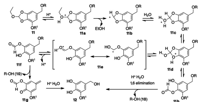
Scheme 3 Proposed mechanism for disassembling of HMPO cargo.
