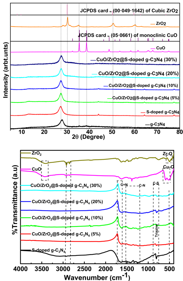
Fig. 2 XRD pattern (top) and FT-IR (bottom) of g\text{-C}_3\text{N}_4 and S-doped g\text{-C}_3\text{N}_4 , \text{CuO}/\text{ZrO}_2@S\text{-doped } g\text{-C}_3\text{N}_4 (5, 10, 20, and 30%) NCs, pure CuO and pure \text{ZrO}_2 NPs.
