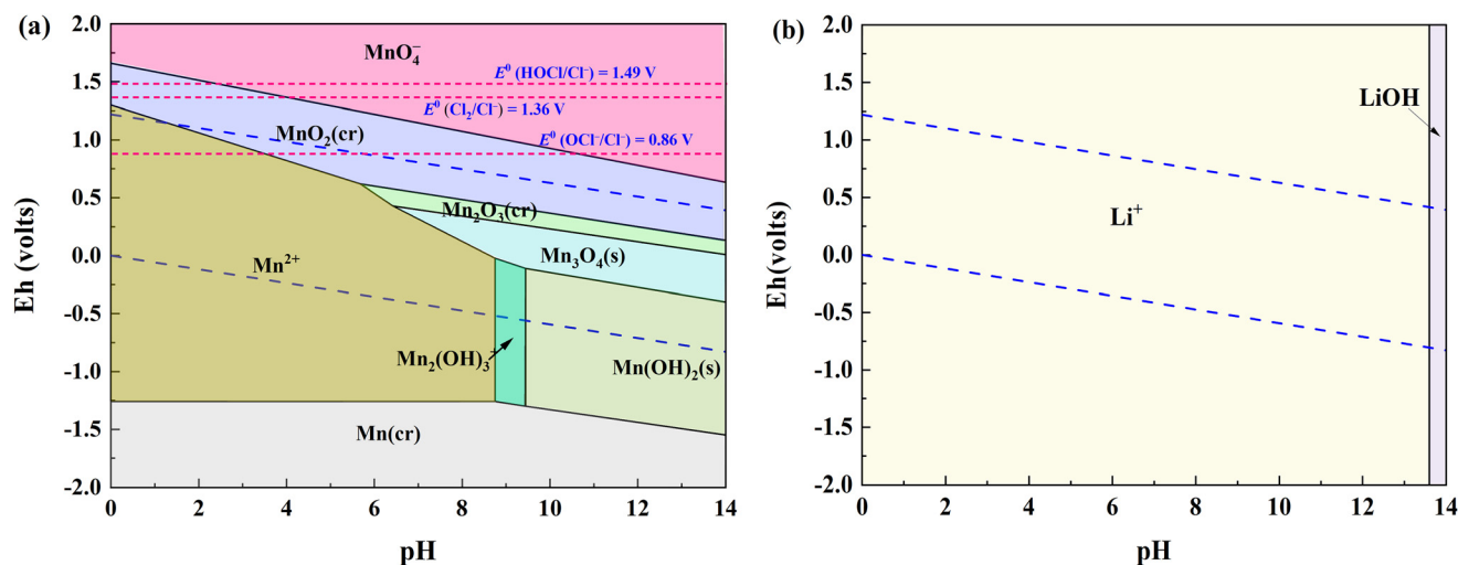
Fig. 2 E_{\text{h}} -pH diagram for the (a) Mn-H 2 O system and (b) Li-H 2 O system ( T = 298.15 K, the molar concentration of Mn and Li was fixed at 1 \times 10^{-3} mol \text{L}^{-1} and 0.1 mol \text{L}^{-1} , respectively).
