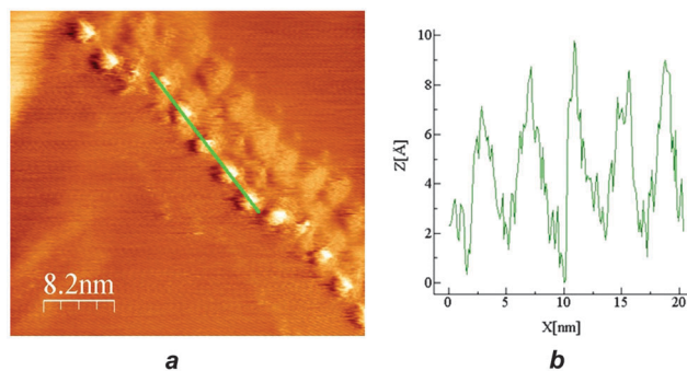
Fig. 1 (a) STM image of a representative chain of beads from [\text{Fe}(\text{bpp})_2]_2[\text{BF}_4]_2 drop cast onto HOPG, with widths of 2.5 nm and heights of 7 \text{\AA} . (b) Profile over the five beads highlighted in (a).
