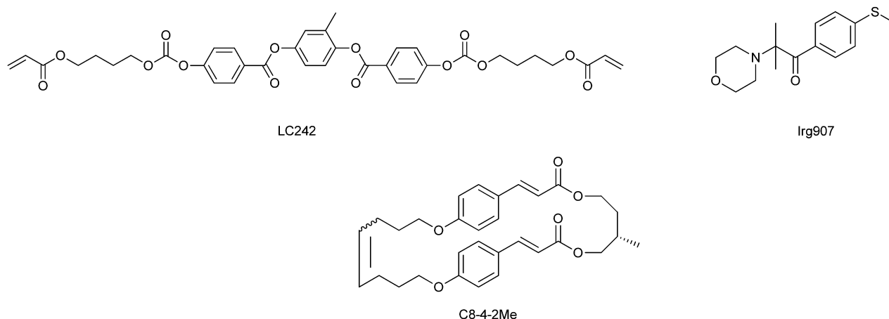
Fig. 1 Chemical structures of the mesogenic compound (LC242), the photoinitiator (PI), and the photoreactive chiral dopant (C8-4-2Me).
