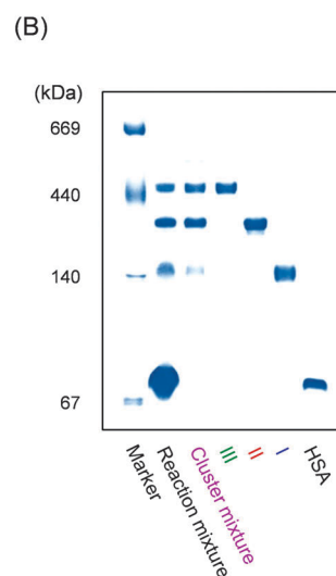
Fig. 2 (A) SEC profiles of the reaction mixture of HbA and HSA (black dotted line), purified HbA-HSA 4 (green line), HbA-HSA 3 (red line), HbA-HSA 2 (blue line), and the cluster mixture HbA-HSA 3 (purple line). (B) The native-PAGE results of the same samples: I, HbA-HSA 2 ; II, HbA-HSA 3 ; III, HbA-HSA 4 .
