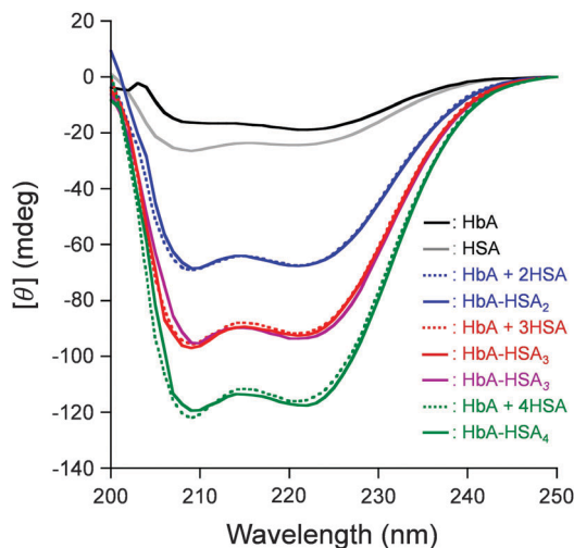
Fig. 3 CD spectra of HbA-HSA m ( m = 2, 3, 4 ), HbA-HSA 3 , HbA, and HSA (0.2 \mu M) in PBS solution (pH 7.4) at 25 °C.
