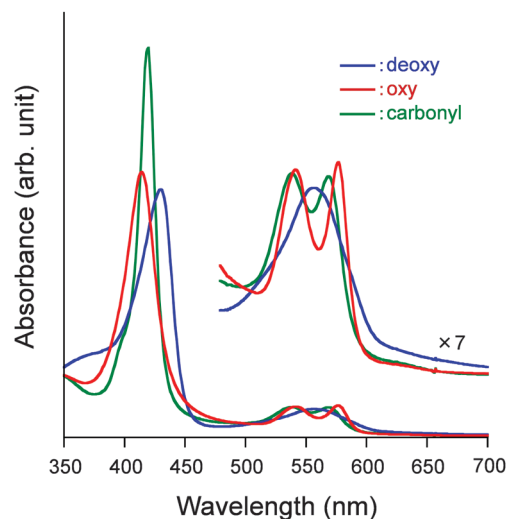
Fig. 5 Visible absorption spectral changes of the HbA-HSA 3 clusters in PBS solution (pH 7.4) at 25 °C.
