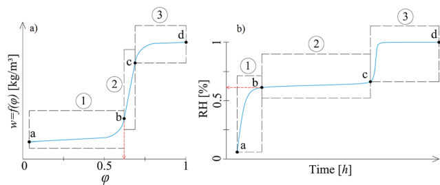
Fig. 2 (a) Schematic representation of a water vapour sorption isotherm portions at different EMC stages a–b, b–c and c–d. (b) Corresponding water vapour sorption kinetics at different EMC stages a–b, b–c and c–d that shows EMC in the segments 1, 2 and 3.
