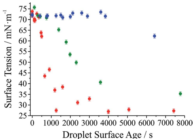
Fig. 5 Surface tension of dilute sodium chloride droplets held in the trapping cell for varying lengths of time. Red circles correspond to measurements where no gas flow was introduced to the cell. Green circles correspond to a gas flow at 80 \text{ mL min}^{-1} using a high purity \text{N}_2 cylinder. Blue circles correspond to a gas flow at the same flow rate but using the boil-off flow from a liquid \text{N}_2 dewar.
