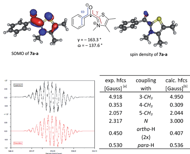
Fig. 1 Top: Plotted SOMOs and spin densities for the postulated key intermediate 7a-a (B3LYP/6-31G*). Bottom: Experimental EPR spectrum 16 and fitted EPR spectrum 17 ( r^2 = 0.93 ) with tabulated hyperfine coupling constants. [a] WINSIM version 0.98. [b] B3LYP/EPR-II//B3LYP/6-31G* for C, H, O, N and 6-31G* for S, Br.
