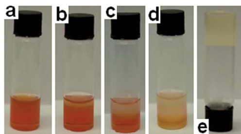
Fig. 7 Organogel containing (a) DMSO (1 mL); 3 (12 mg mL -1 ) and 6 (10 mg mL -1 ); (b) 60 seconds after DCP (0.1 mL) addition; (c) 25 min after DCP addition; (d) 60 min after DCP addition; (e) 22 h after DCP addition. Temperature maintained at approximately 21 °C.
