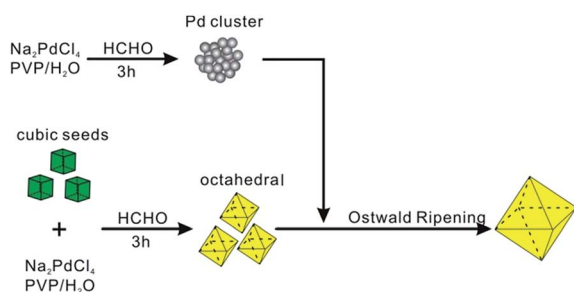
Fig. 1 Schematic illustration of Ostwald ripening in a bimodal-sized Pd colloidal system.
