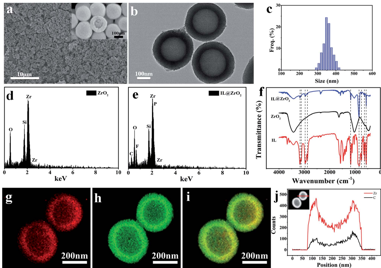
Fig. 1 Characterization of the physicochemical properties of the multifunctional IL@ZrO 2 nanoparticles. (a) Low (×5k) and high (×100k, inset) magnification SEM images, (b) TEM image, and (c) histogram of the distribution of diameters of the IL@ZrO 2 nanoparticles. The histogram of the distribution of diameters was based on statistical analysis of the results via measuring the size of 100 nanoparticles in (a). EDX spectra of (d) the hollow ZrO 2 nanoparticles and (e) the multifunctional IL@ZrO 2 nanoparticles. (f) FT-IR spectra of the ZrO 2 nanoparticles, multifunctional IL@ZrO 2 nanoparticles and IL. STEM-EDX spectral element mapping for (g) carbon and (h) zirconium. (i) Merged overlay image formed from (g) and (h), showing the clear structure. (j) Cross sectional compositional line profiles of IL@ZrO 2 .
