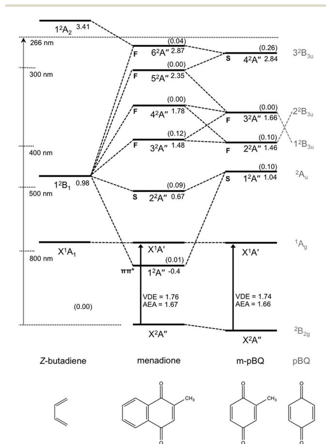
Fig. 6 Energy level and correlation diagram of calculated electron excitation and detachment energetics for Z-butadiene, menadione, and m-pBQ. For m-pBQ, the corresponding resonances in pBQ are noted in grey. 'S' and 'F' indicate shape and Feshbach resonances, respectively. Calculated dipole transition oscillator strengths are given in parentheses. VDE is the vertical detachment energy and AEA is the adiabatic electron affinity. All energies are given in units of eV, and uncertainty in the calculated energetics are estimated at \pm 0.15 eV.
