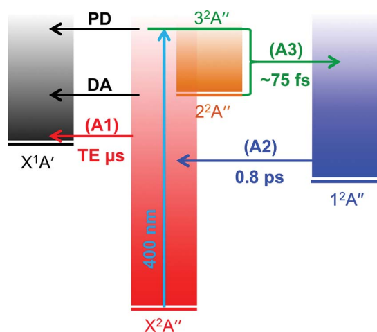
Fig. 8 Schematic summary of menadione temporary anion dynamics following absorption of a 3.10 eV (400 nm) photon. A1, A2, and A3 are the three pump-probe features identified in the time-resolved imaging experiments, and DA is the small contribution of delayed autode-tachment identified in the frequency- and angle-resolved imaging experiments. TE corresponds to thermionic emission, which is the predominant electron loss channel.
