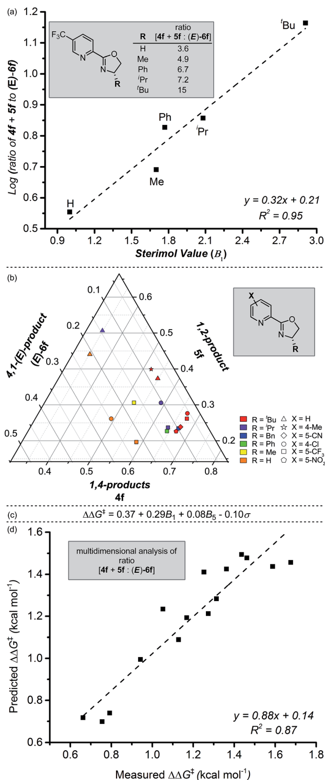
Fig. 3 (a) Correlation between site selectivity of alkene insertion and Sterimol B_1 values. (b) Ternary plot of normalized isomeric product distribution resulting from pyrox ligand screen. (c) Normalized mathematical relationship describing differential free energy of alkene insertion selectivity. (d) Predicted versus measured \Delta\Delta G^\ddagger plot derived from Sterimol B_1 values, Sterimol B_5 values, and Hammett \sigma values for site selectivity of alkene insertion.
