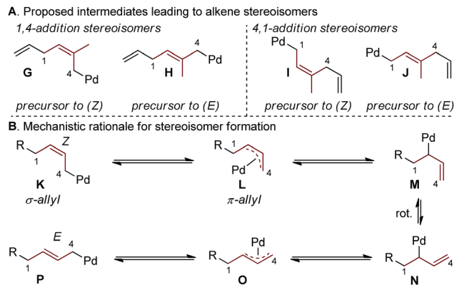
Fig. 2 Rationale accounting for stereoisomer formation.
