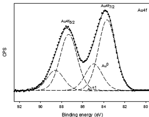
Fig. 8 XPS spectra in the Au 4f region of Au@UiO-66-NaBH 4 after catalysis.
