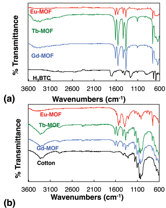
Fig. 7 FTIR spectra of (a) H 3 BTC and Ln-MOFs solids, and (b) clean cotton and Ln-MOFs grown on cotton fibers.
