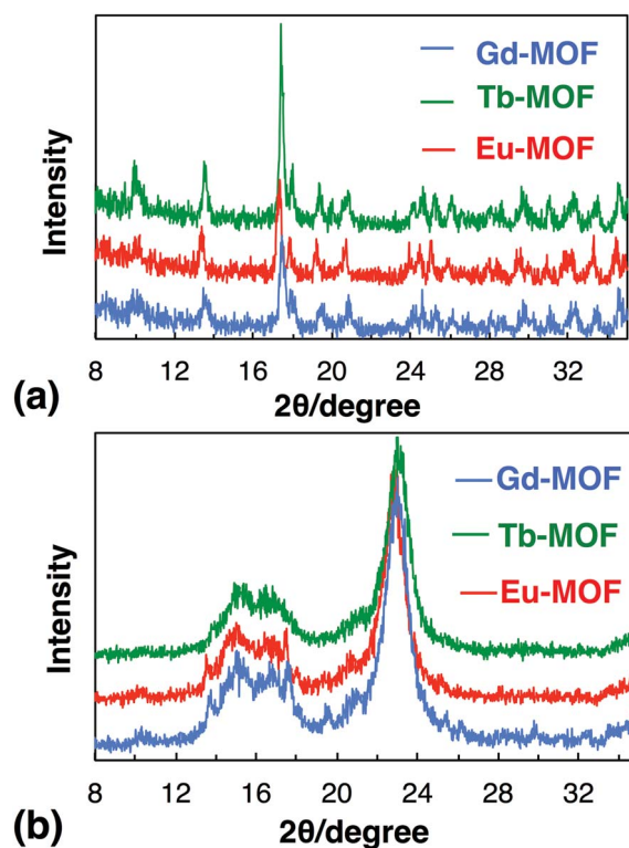
Fig. 6 PXRD patterns of Ln-MOFs (a) solids collected after the growth (b) grown on cotton fibers.
