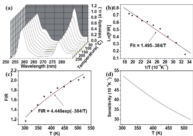
Fig. 5 Temperature dependent (a) spectrum of \text{Er}^{3+} ions from {}^4\text{D}_{7/2} and {}^4\text{G}_{9/2} levels; (b) log plot of the FIR; (c) FIR relative to the temperature; and (d) sensor sensitivity under 980 nm excitation. Reprinted from ref. 38 with permission of Optical Society of America.
