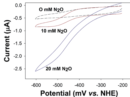
Fig. 4 The effect of \text{N}_2\text{O} concentration on the voltammetric response from CoMb. Methyl viologen (40 \mu\text{M} ) was used as the mediator with a scan rate of 5 mV \text{s}^{-1} . \text{N}_2\text{O} concentration was varied by adding aliquots of a mediator solution saturated with \text{N}_2\text{O} .
