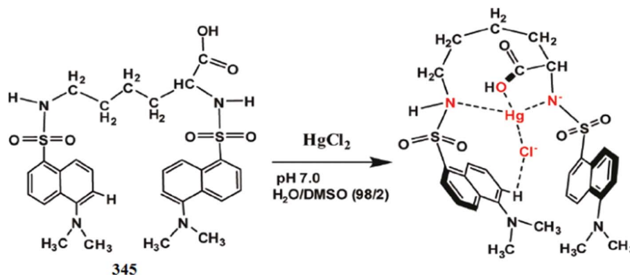
Fig. 305 Chemical structure of ligand 345 and the proposed binding mode toward Hg 2+ .
