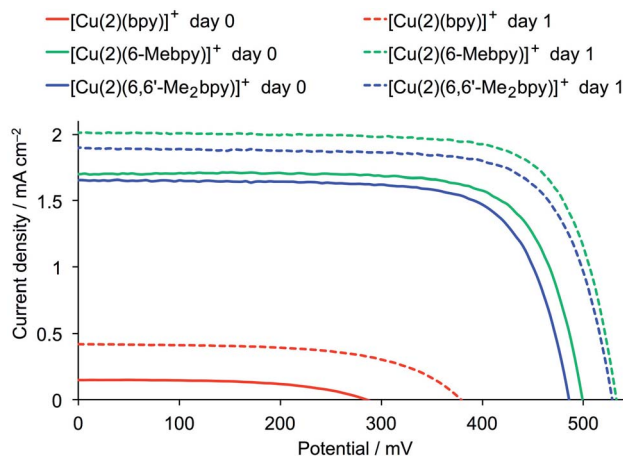
Fig. 3 J - V curves for DSCs with the dyes [Cu(2)(bpy)] + , [Cu(2)(6-Mebpy)] + and [Cu(2)(6,6'-Me 2 bpy)] + measured on the day of sealing the DSC and one day later.
