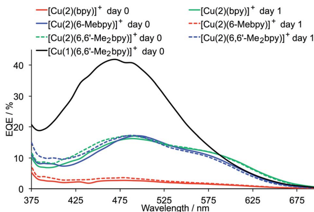
Fig. 4 EQE spectra for DSCs with the dyes [Cu(2)(bpy)] + , [Cu(2)(6-Mebpy)] + and [Cu(2)(6,6'-Me 2 bpy)] + measured on the day of sealing the cell and one day later, and with [Cu(1)(6,6'-Me 2 bpy)] + measured on the day of sealing.
