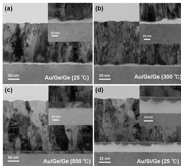
Fig. 1 Cross-sectional HRTEM images of the interface morphology in Au/Ge/Ge and Au/Si/Ge samples prepared at different temperatures. The insets show higher-resolution images of the interface morphology.
