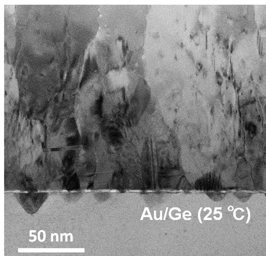
Fig. 3 Cross-sectional HRTEM images of the interface morphology in the Au/c-Ge sample prepared at 25 °C.
