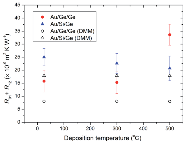
Fig. 2 Measured TBR at two interfaces in Au/Ge/Ge and Au/Si/Ge three-layer samples as a function of deposition temperature. DMM-predicted values are plotted for comparison.
