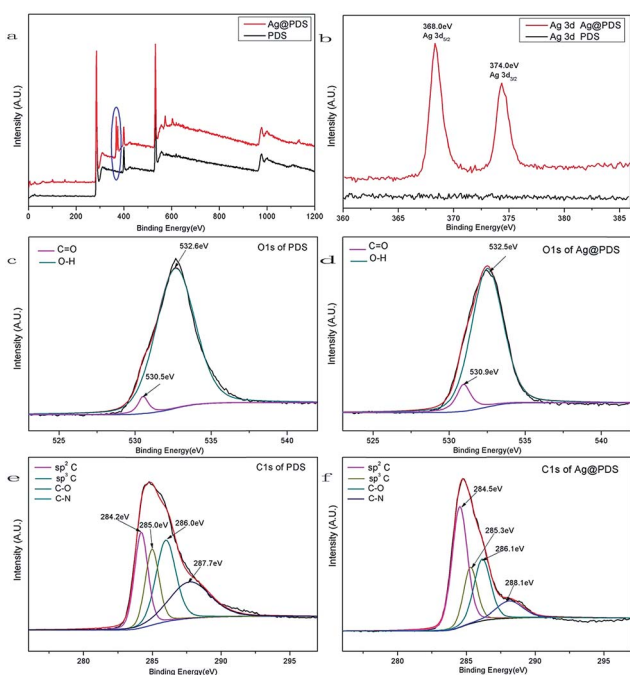
Fig. 6 X-ray photoelectron spectra (XPS) of (a) scan survey, (b) Ag3d, (c) and (d) O1s, (e) and (f) C1s of poly-dopamine spheres (PDS) and poly-dopamine spheres loaded with silver nanoparticles (Ag@PDS).
