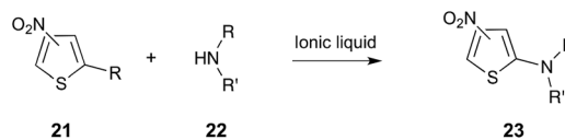
Scheme 9 The nucleophilic aromatic substitution reaction between the substituted thiophenes 21 and a number of cyclic, secondary amines 22 (for example, R/R' = -(\text{CH}_2)_4- , -(\text{CH}_2)_5- , -(\text{CH}_2)_2\text{O}(\text{CH}_2)_2- ). 27,282
